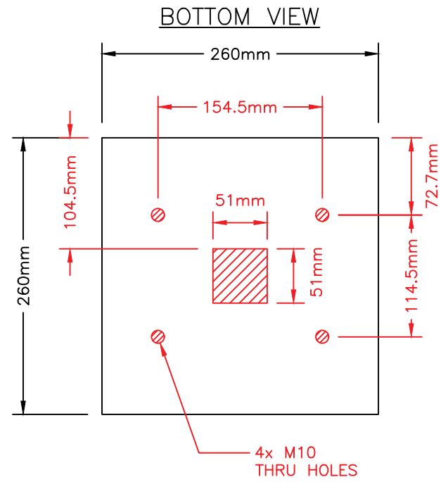
BASEPLATE CUT-OUT DETAILS (4mm THICK)
